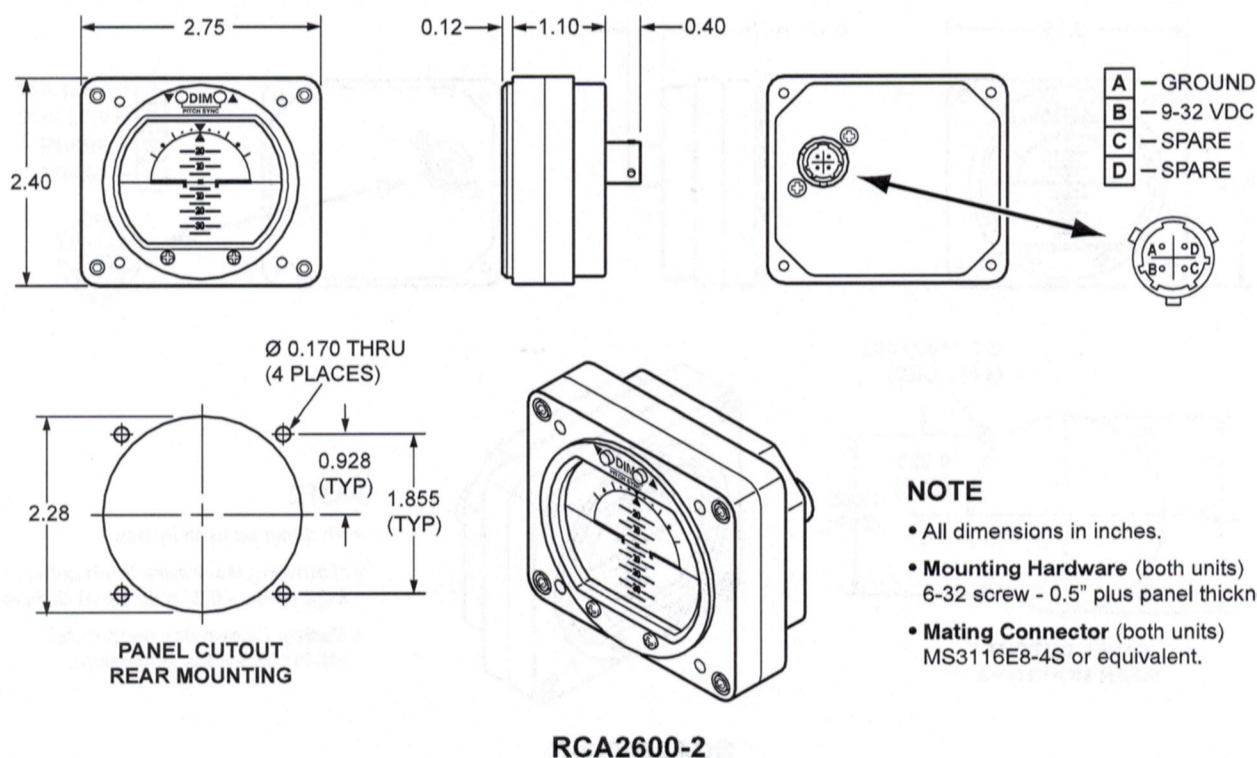
Figure 1.1, General Dimensions
