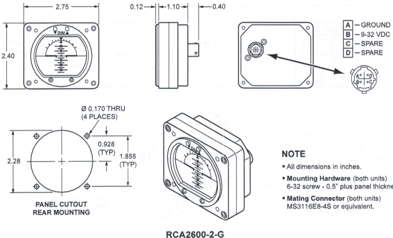
Figure 1.2, General Dimensions (-G Models)
