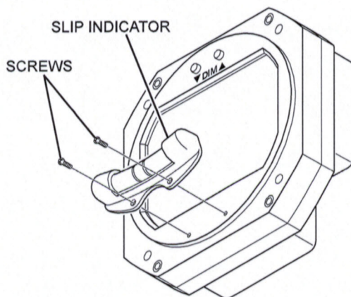
Figure 4.1, Inclinometer Installation
